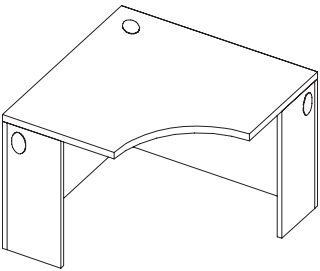
Curved Front Corner Surface Full Modesty, 1” Thick Surface
