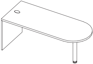
D-Table, 1.5" Thick Surface
