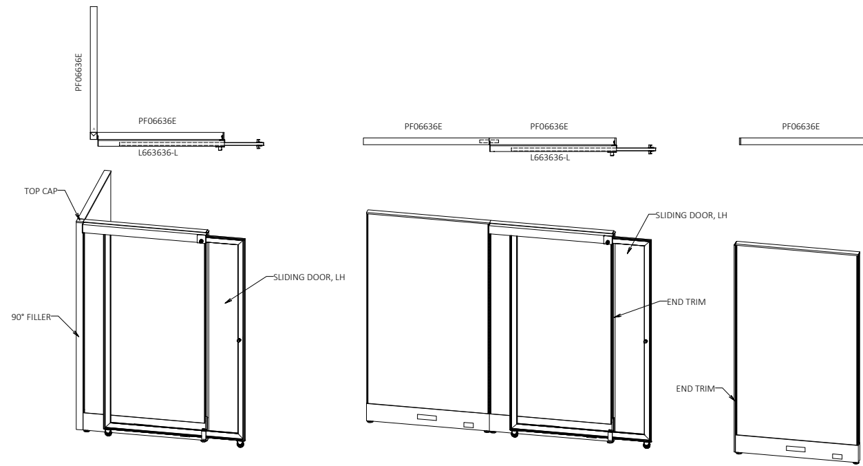
2-Way 90° Connection
