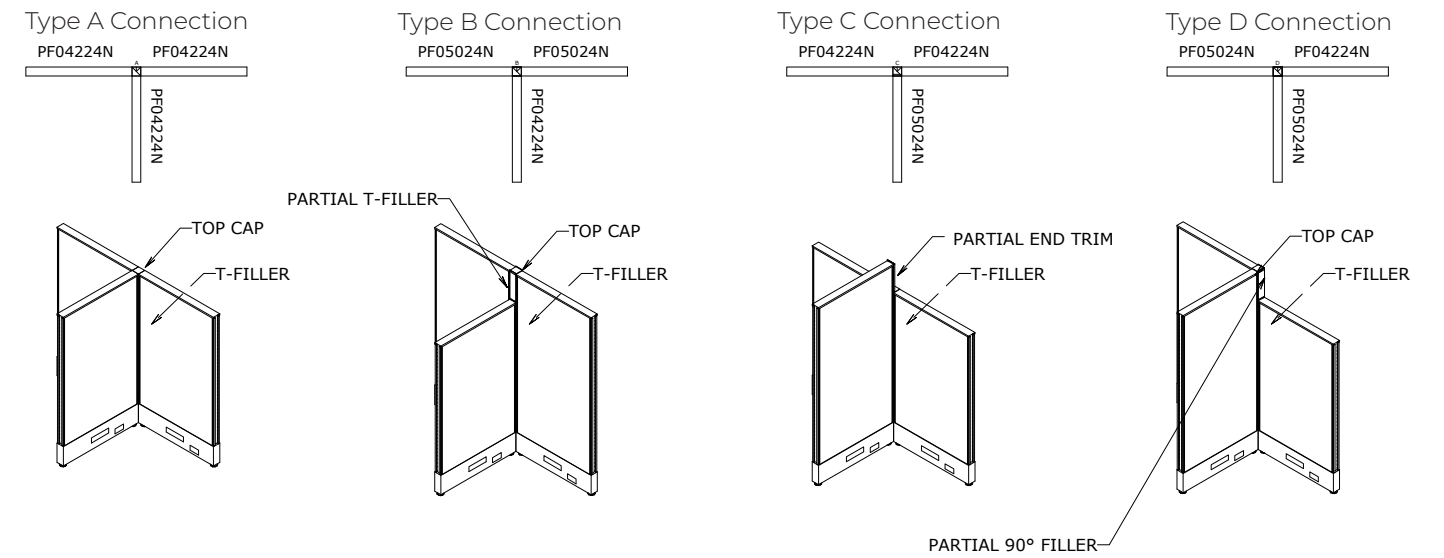
3-Way Connection
