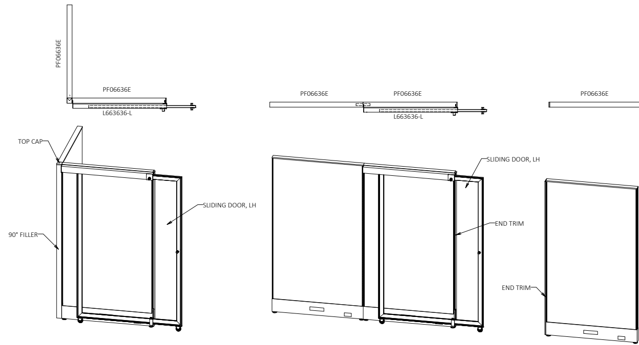
2-Way 90° Connection
