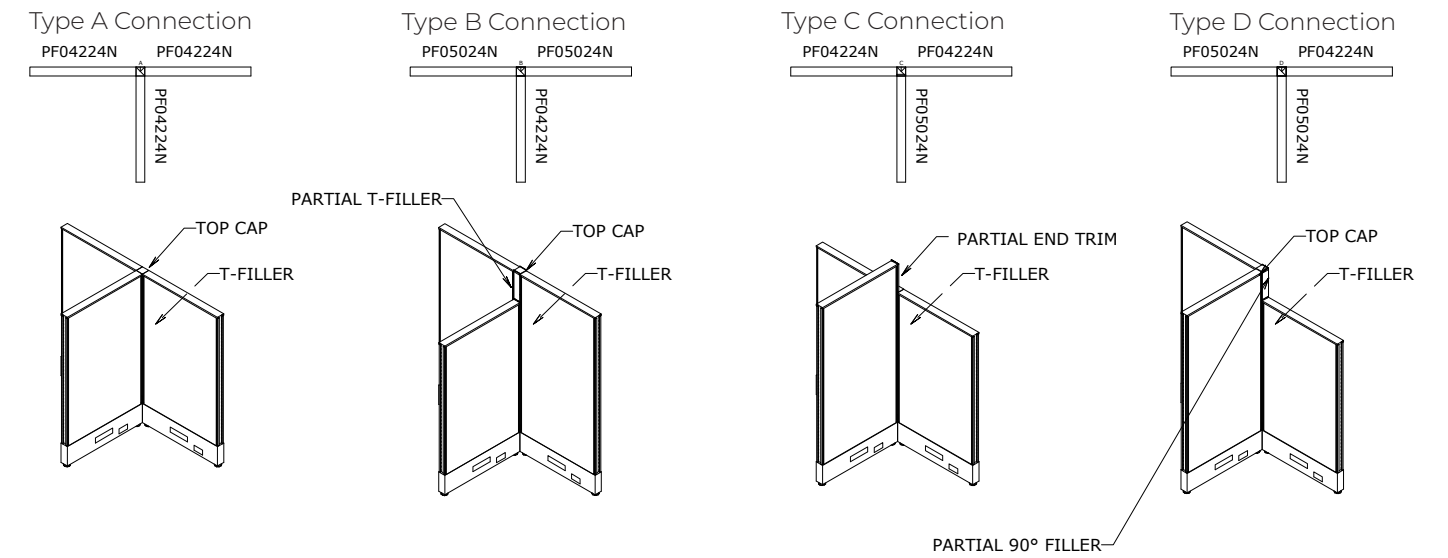
3-Way Connection
