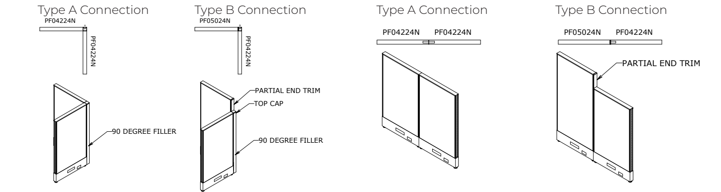
2-Way 90° Connection
