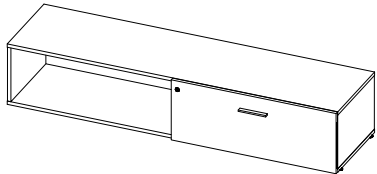
TL-CRLS Credenza w/ Lateral File LH, Storage Cabinet RH W: 72" D: 21"- 24" H: 29"
