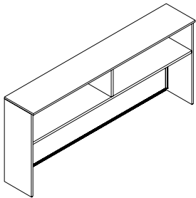
M-SH00 Open Hutch 3/4" Thick W: 30" - 84" D: 15" H: 38"
