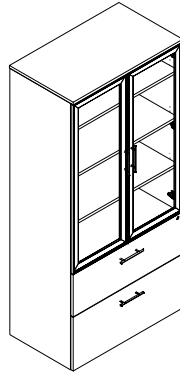
MB-FCSL-G Combo Cabinet with Storage & Lateral Files and Acrylic Doors 3/4" thick top W: 36" D: 21" H: 78"
