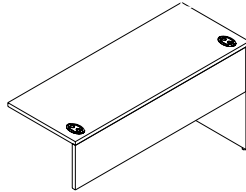
ML-WS1Z [L,R,C,D]-L / ML-WS1Z [L,R,C,D]-R Straight w/ Partial Modesty (Left Hand shown) W: 24"- 60" D: 21"- 30" H: 29"
