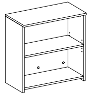
M-SHWO Open Hutch 3/4" Thick W: 15" D: 24" - 48" H: 30"
