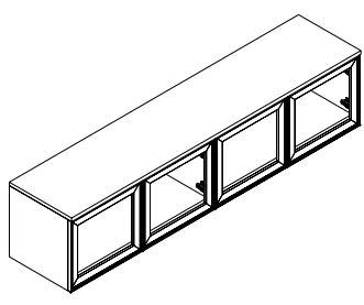
M-SHHW-G Wall Mounted Hinged Door Hutch w/ Acrylic Doors 3/4" Thick W: 30" - 72" D: 15" H: 16.5"
