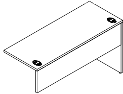
M-WS1Z [L,R,C,D]-L / M-WS1Z [L,R,C,D]-R Straight w/ Partial Modesty (Left Hand shown) W: 24"- 60" D: 21"- 30" H: 29.5"
