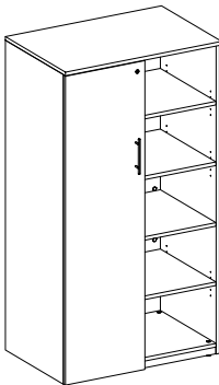
M-FTSO-L/ M-FTSO-R Open & Closed Combo Tower 3/4" Thick (Left Hand shown) W: 24"-36" D: 24" H: 53"- 68"
