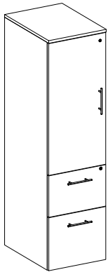
ML-FCWF-L/ ML-FCWF-R Freestanding Combo cabinet FF W: 18" D: 24" H: 67"
