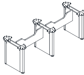
MB-B5 Elliptical Base for Straight/Boat Tabletop W: 36" - 60" D: 72" - 204" H: 28"
