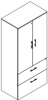
ML-FCSL Freestanding Combo Lateral Storage Double Door 3/4" Thick W: 36" D: 21" H: 67"
