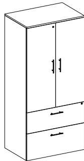
M-FCWL-L/ M-FCWL-R Lateral Combo Cabinet Wardrobe 3/4" Thick (Left Hand shown) W: 30"-36" D: 24" H: 67"
