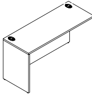
ML-WS1G [L,R,C,D]-L / ML-WS1G [L,R,C,D]-R Straight w/ Full Modesty (Left Hand shown) W: 24"- 60" D: 21"- 30" H: 29"
