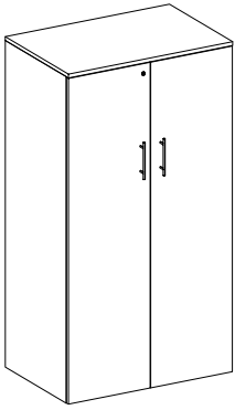
ML-FSDB-L/ML-FSDB-R Wardrobe Tower 3/4" Thick (Left Hand shown) W: 12"-36" D: 24" H: 67"
