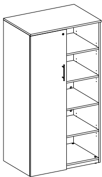
ML-FTSO-L/ML-FTSO-R Open & Closed Combo Tower 3/4" Thick (Left Hand shown) W: 67" D: 24" H: 67"
