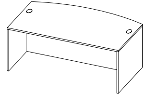
TL-TARG Arc w/ Full Recessed Modesty W: 72"- 96" D: 36" H: 29"
