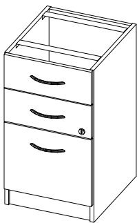
T-FPBU-X Underdesk Box/Box/File Full Back W: 16" D: 18" - 24" H: 28"
