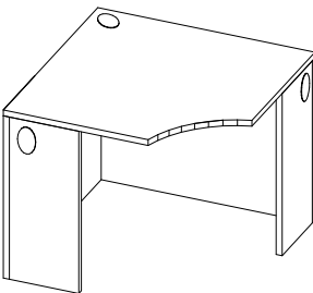
TL-W5C0 Curve Front Full Modesty w/ Intermediate Gable W: 36" - 42" D: 21" - 24" H: 29"
