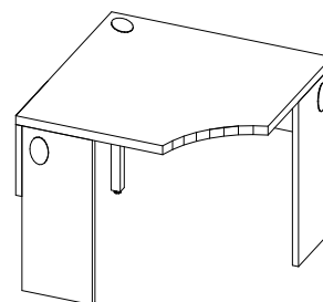
T-W5C0-P Curve Front Partial Modesty w/ Intermediate Gable W: 36" - 42" D: 21" - 24" H: 29.5"
