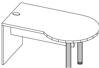
T-TFSG-L / T-TFSG-R F-Table (Left Hand shown) W: 60"- 84" D: 24" H: 29.5"
