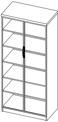
TB-FSDS-G Double Door Storage Cabinet with Shelves and Acrylic Doors W: 36" D: 21" H: 78"
