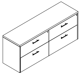
M-CRLL Credenza w/ Double Lateral Files W: 72" D: 21" - 24" H: 29.5"
