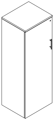
ML-FSDC-L / ML-FSDC-R Freestanding Wardrobe Tower 3/4" Thick (Left Hand shown) W: 24" D: 21" H: 67"
