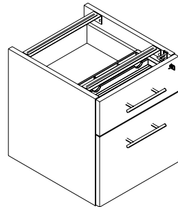
M-FPSU Suspended Box/File W: 16" D: 18" H: 16"
