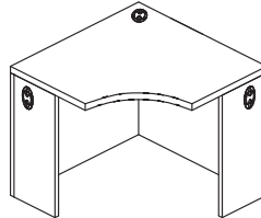
ML-W5C0 Curved Front Full Modesty w/ Intermediate Gable W: 36"- 42" D: 21"- 24" H: 29"
