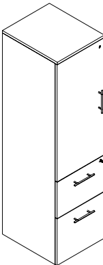
M-FCSF-L / M-FCSF-R Combo Cabinet w/Storage and File/File 3/4" Thick (Left Hand shown) W: 18" D: 21" H: 68"
