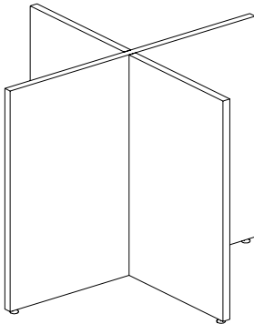
M-B6 Cross Base W: 18" - 48" D: 18" - 48" H: 28"
