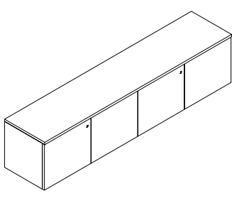
M-SHHW-L Wall Mounted Hinged Door Hutch 3/4" Thick W: 30" - 72" D: 15" H: 16.5"
