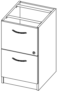
T-FPFU-X Underdesk File/File Full Back W: 16" D: 18" - 24" H: 28"
