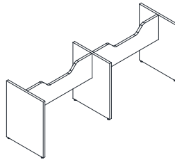
QMB-B4-R Gable Base for Racetrack Tabletop W: 48" - 60" D: 84" - 240" H: 28"
