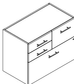
M-FPJU-L / M-FPJU-R Underdesk Combo Pedestal w/Box/Box/File and File/File LH/ RH (LH shown) W: 36" D: 20" - 21" H: 28"
