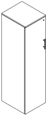
M-FSDS-L / M-FSDS-R Freestanding Storage Tower 3/4" Thick (Left Hand shown) W: 18" D: 21" H: 68"
