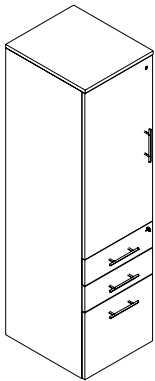
ML-FCSB-L / ML-FCSB-R Combo Cabinet w/Storage and Box/Box/File 3/4" Thick (Left Hand shown) W: 18" D: 21" H: 67"
