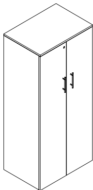
M-FSDS Freestanding Storage Tower Double Door 3/4" Thick W: 36" D: 21" H: 68"
