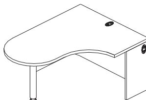
ML-TJ0G-L / ML-TJ0G-R J-Table (Left Hand shown) W: 60"- 84" D: 24" H: 29"
