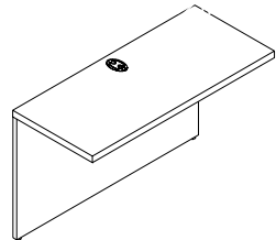
M-BS0G Straight w/ Full Modesty W: 30" - 48" D: 21" - 24" H: 29.5"
