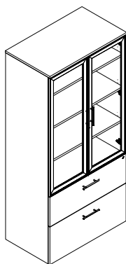
MB-FCSL-G Combo Cabinet with Storage and Lateral Files and Acrylic Doors 3/4" thick top W: 36" D: 21" H: 78"
