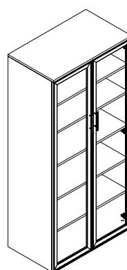
MB-FSDS-LG / MB-FSDS-RG Storage Cabinet with Shelves and Acrylic Doors (Left Hand shown) W: 18" D: 21" H: 78"
