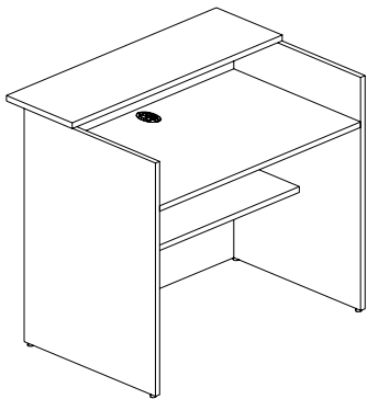
ML-RCWG-S Service Write Up Desk w/ Straight Countertop W: 30 - 84" D: 30" H: 43"
