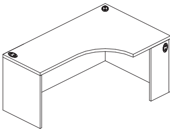
M-UC4G-L / M-UC4G-R Unitized Desk (Left Hand shown) Full Modesty w/ Full & Partial Gable W: 66" - 72" D: 39" - 42" Other D: 21" - 24" H: 29.5"
