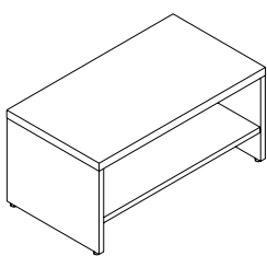
M-TCTS Coffee Table with Fixed Shelf W: 36" D: 20" H: 17.5"
