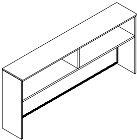
M-SHO0 Open Hutch 3/4" Thick W: 30" - 84" D: 15" H: 38"
