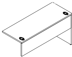
ML-WS1Z-L / ML-WS1Z-R Straight w/ Partial Modesty (Left Hand shown) W: 24" - 60" D: 21" - 30" H: 29"
