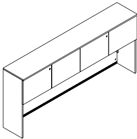
M-SHH0 Hinged Door Hutch 3/4" Thick W: 30" - 84" D: 15" H: 38.5"
