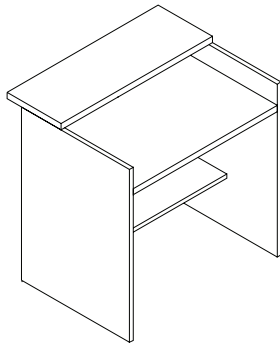
M-RCWG-S Service Write Up Desk w/ Straight Countertop W: 30 - 84" D: 30" H: 43"
