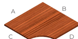
5 Corner Curved Worksurface with Right Hand Cropped Depth A: 35" - 47" B: 36" - 48" C: 24" - 30" D: 23" - 29"
