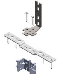
L-HC3W-C 3 Way C Panel Connector
