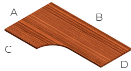
L-WUCO Unitized Curved Worksurface with Side A Cropped Depth A: 35" B: 54" - 96" C: 24" D: 23" RH Shown
