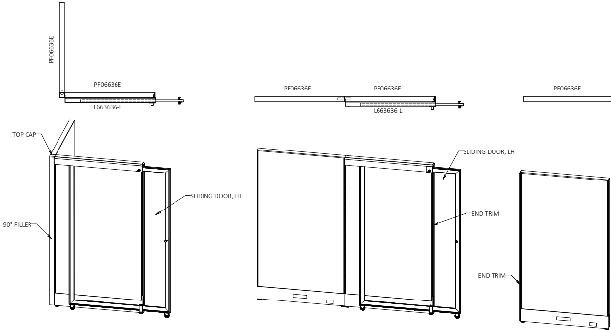
2-Way 90° Connection
