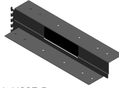
L-HSSE-P Return Support Standard Mount with Power H: 3" W: 24", 30"
