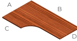
Unitized Curved Worksurface with Side B Cropped Depth A: 36" B: 53" - 95" C: 23" D: 24" RH Shown
