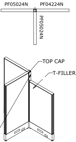
Type D Connection
