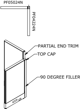
Type B Connection
