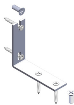
QL-HC2W-180-B 180 Degree B Panel Connector
