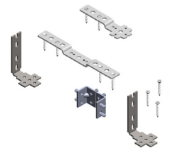
QL-HW2/QL-HW4/QL-HW6 Wall Connector H: 34", 42", 50", 66", 82" W: 2", 4", 6"
