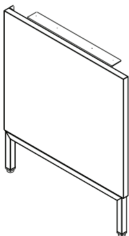
Gallery Panel Wrap Laminate Gable
