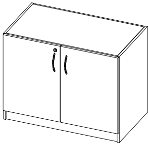
T-FSU0 Underdesk Storage Cabinet W: 30" - 42" D: 19" - 21" H: 28"
