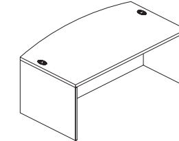
QML-TARG Arc w/ Full Recessed Modesty W: 72" - 96" D: 36" H: 29"
