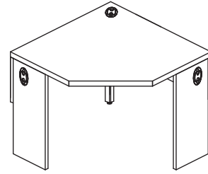
QML-W5S0-P Straight Front Partial Modesty w/ Intermediate Gable W: 36" - 42" D: 21" - 24" H: 29"
