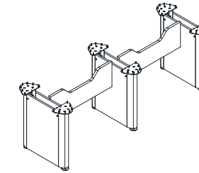
QMB-B5-R Elliptical Base for Racetrack Tabletop W: 48" - 60" D: 84" - 240" H: 28"
