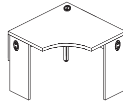
QML-W5C0-P Curve Front Partial Modesty w/ Intermediate Gable W: 36" - 42" D: 21" - 24" H: 29"
