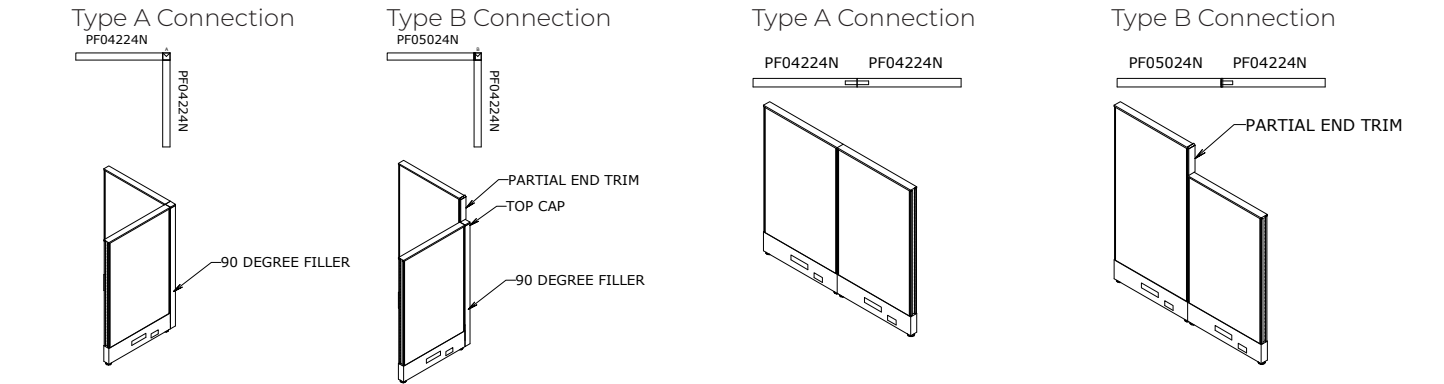
2-Way 90° Connection
