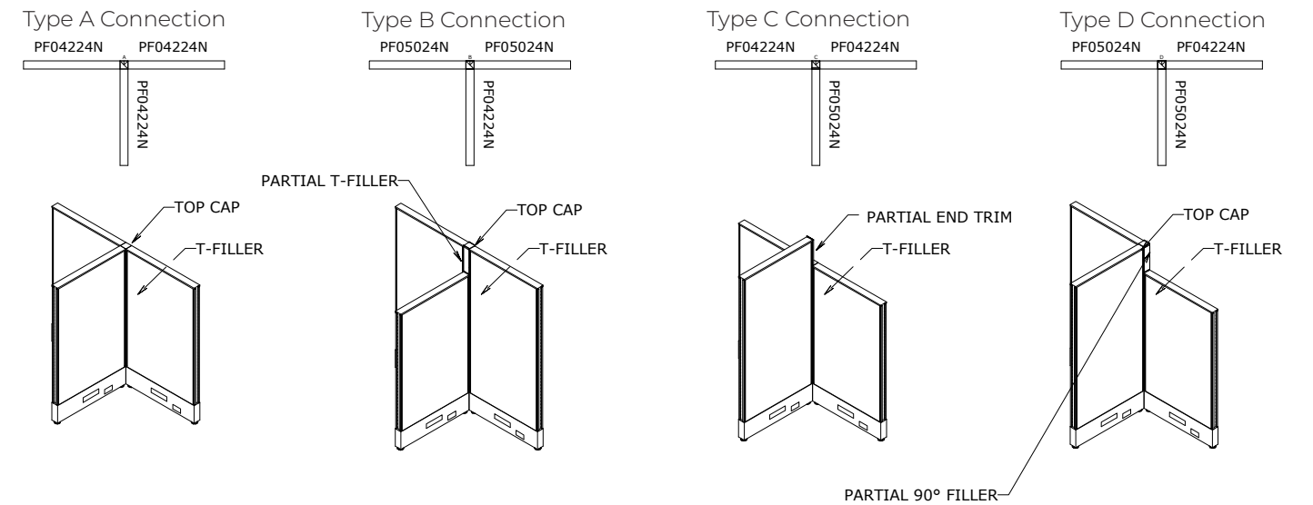
3-Way Connection
