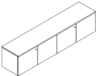
QML-SHHW-L Wall Mounted Hinged Door Hutch W: 30" - 72" D: 15" H: 16.5"
