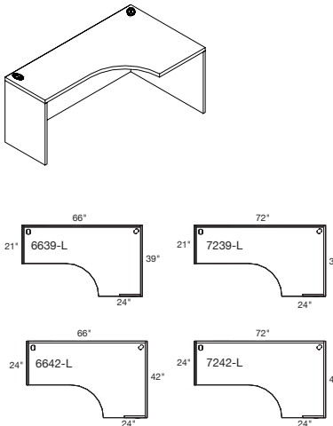
1" Curved Front Unitized Desk w/Full Modesties, No Gables LH Shown
