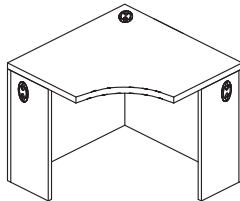
QML-W5C0 Curve Front Full Modesty w/ Intermediate Gable W: 36"- 42" D: 21"- 24" H: 29"
