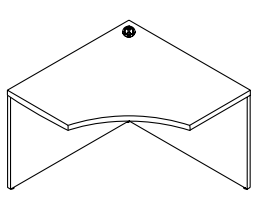
M-W5C0-N Curve Front Full Modesty/ No Gable W: 36"- 42" D: 21"- 24" H: 29.5"
