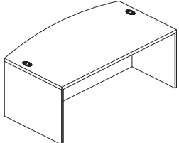
M-TARG Arc w/ Full Recessed Modesty W: 72"- 96" D: 36" H: 29.5"
