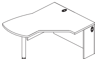
ML-TFSG-L / ML-TFSG-R F-Table (Left Hand shown) W: 60"- 84" D: 24" H: 29"
