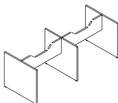
QMB-B4-R Gable Base for Racetrack Tabletop W: 48" - 60" D: 84" - 240" H: 28"
