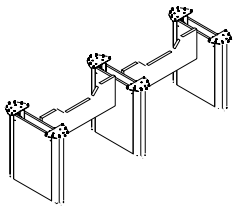
QMB-B5 Elliptical Base for Straight/ Boat Tabletop W: 30" - 60" D: 72" - 240" H: 28"
