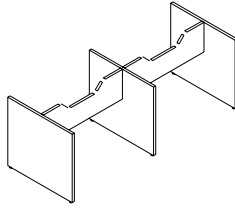
QMB-B4-T Gable Base for Tapered Tabletop W: 48" - 240" D: 84" - 240" H: 28"
