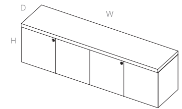
Hinged Door Overhead Storage, 1" Thick Top
