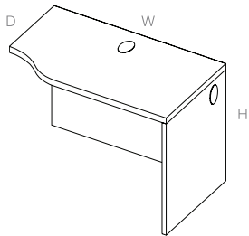
Bowed Return Full Modesty, 1” Thick Surface
