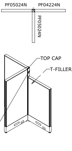
Type D Connection
