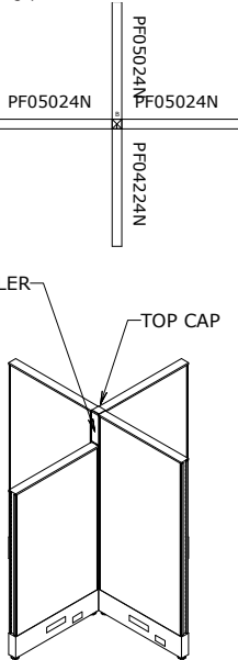
Type B Connection
