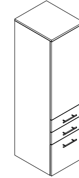
M-FCSB-L / M-FCSB-R Combo Cabinet w/Storage and Box/Box/File 3/4" Thick (Left Hand shown) W: 18" D: 21" H: 68"
