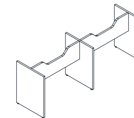
MB-B4-R Gable Base for Racetrack Tabletop W: 48" - 60" D: 84" - 240" H: 28"
