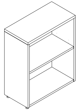
ML-SBOX Bookcase 3/4" Thick W: 24" - 42" D: 12"/15"/21" H: 29"/67"/77"
