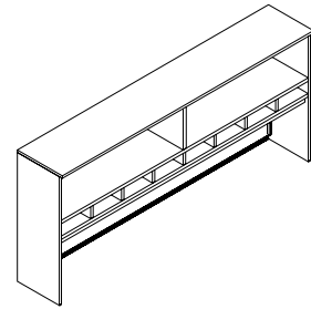
M-SH0P Open Hutch w/ Pigeon Holes 3/4" Thick W: 30" - 84" D: 15" H: 38.5"
