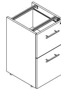
M-FPFU Underdesk File/File W: 16" D: 18" - 24" H: 28"
