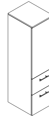
M-FCSF-L / M-FCSF-R Combo Cabinet w/Storage and File/File 3/4" Thick (Left Hand shown) W: 18" D: 21" H: 68"
