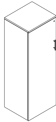
ML-FSDC-L / ML-FSDC-R Freestanding Wardrobe Tower 3/4" Thick (Left Hand shown) W: 24" D: 21" H: 67"
