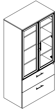
MB-FCSL-G Combo Cabinet with Storage and Lateral Files and Acrylic Doors 3/4" thick top W: 36" D: 21" H: 78"
