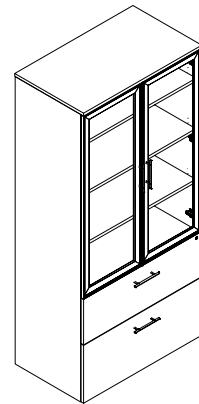
ML-FCSL-G Freestanding Combo Lateral Storage Glazed Double Door 3/4" Thick W: 36" D: 21" H: 67"
