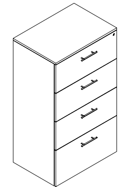
M-FL4F Freestanding 4-Drawer Lateral File 1.5" Thick W: 30" - 36" D: 21" H: 52.5"
