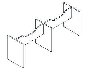
MB-B4-T Gable Base for Tapered Tabletop W: 48" - 78" D: 84" - 240" H: 28"
