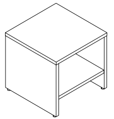
ML-TCTS End Table with Fixed Shelf W: 20" - 30" D: 20" - 30" H: 19"
