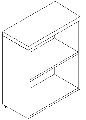
M-SBOX Bookcase 3/4" Thick W: 24" - 42" D: 12"/15"/21" H: 29"/42"/54"/68"/78"
