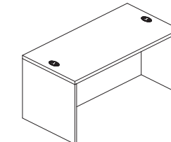
ML-TSRG Straight w/ Full Recessed Modesty W: 60" - 96" D: 30" - 36" H: 29"
