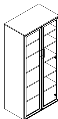
MB-FSDS-LG / MB-FSDS-RG Storage Cabinet with Shelves and Acrylic Doors (Left Hand shown) W: 18" D: 21" H: 78"
