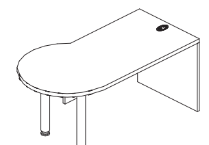
ML-TPOG-L / ML-TPOG-R P-Table (Left Hand shown) W: 60" - 84" D: 30" H: 29"
