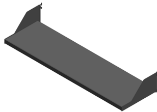
QL-S00M Steel Shelf H: 6" W: 30" - 60" D: 12"
