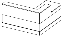
R2-L0TH-XXXX-A-X L-Shape w/ Half Transaction Left hand/Right hand W: 72"-96" D: 72"-96" *Half transaction is always on user side *Right hand shown
