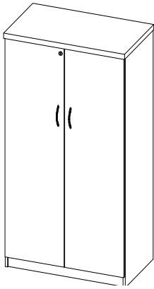
T-FSDS Double Door Storage Cabinet w/ Shelves W: 36" D: 21" H: 68"
