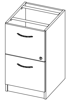
T-FPFU-X Underdesk File/File Full Back W: 16" D: 18" - 24" H: 28"
