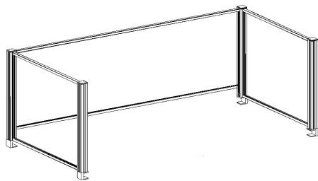
1 front shield
