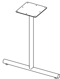
R-HTB-T Tubular T-Base H: 35" D: 16"-34"
