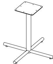
R-HTB-X Tubular X-Base H: 28" D: 16"-48"
