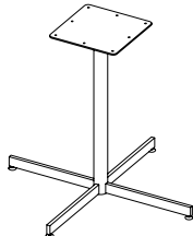
R-HSB-X Slim X-Base H: 21" D: 16"-34"
