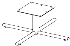
R-HTB-X Tubular X-Base H: 15" D: 16"-48"
