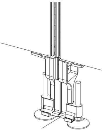
Self-leveling Details
